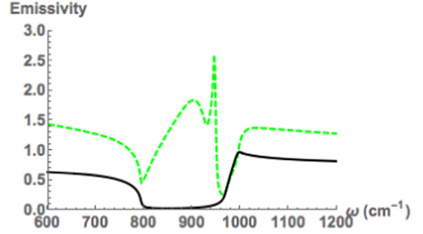
Fig. 2. Emissivity vs angular frequency for a circular aperture filled with SiC with a radius of 100 \mu\text{m} (plain) and with a radius of 10 \mu\text{m} (dashed).
