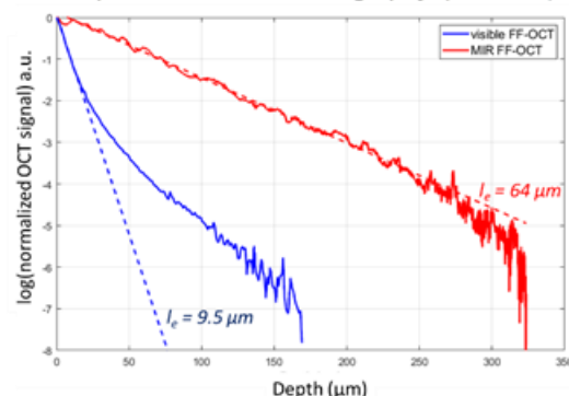
Figure 2: FF-OCT measurement of the extinction mean-free-path l_e of white acrylic paint in the MIR spectral range (MWIR, 3–5 \mu\text{m} ) compared to the same measurement at visible wavelengths.
