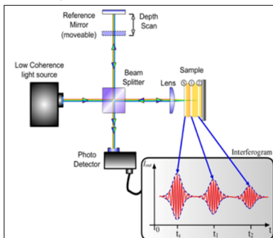
Figure 1: Schematic graph of an early time-domain optical coherence tomography (TD-OCT)
