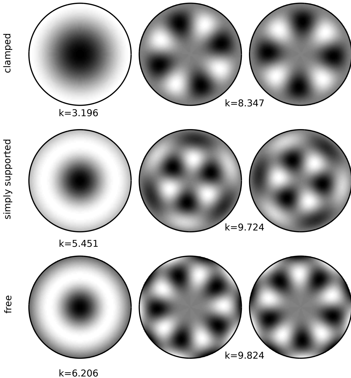
Fig. 3 Some examples of eigenmodes, for simple and double eigenvalues, of the circular plate with clamped, simply supported and free boundary conditions
