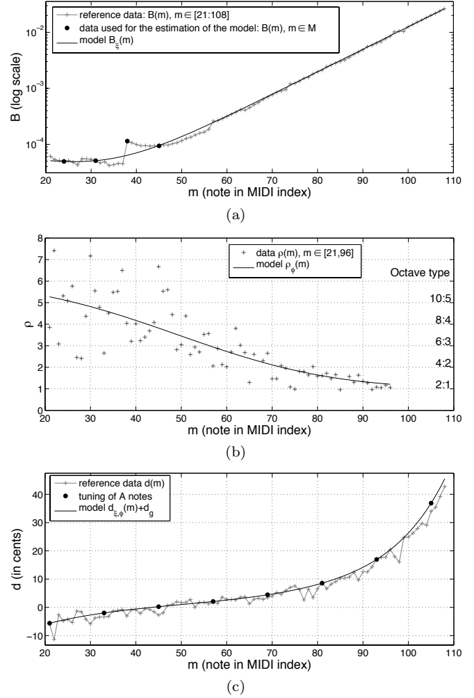
FIG. 8. RWC grand piano #2. (a) Inharmonicity coefficient B , (b) octave type parameter \rho , (c) deviation from ET along the whole compass. The data are depicted as grey '+' markers and the model as black lines.
