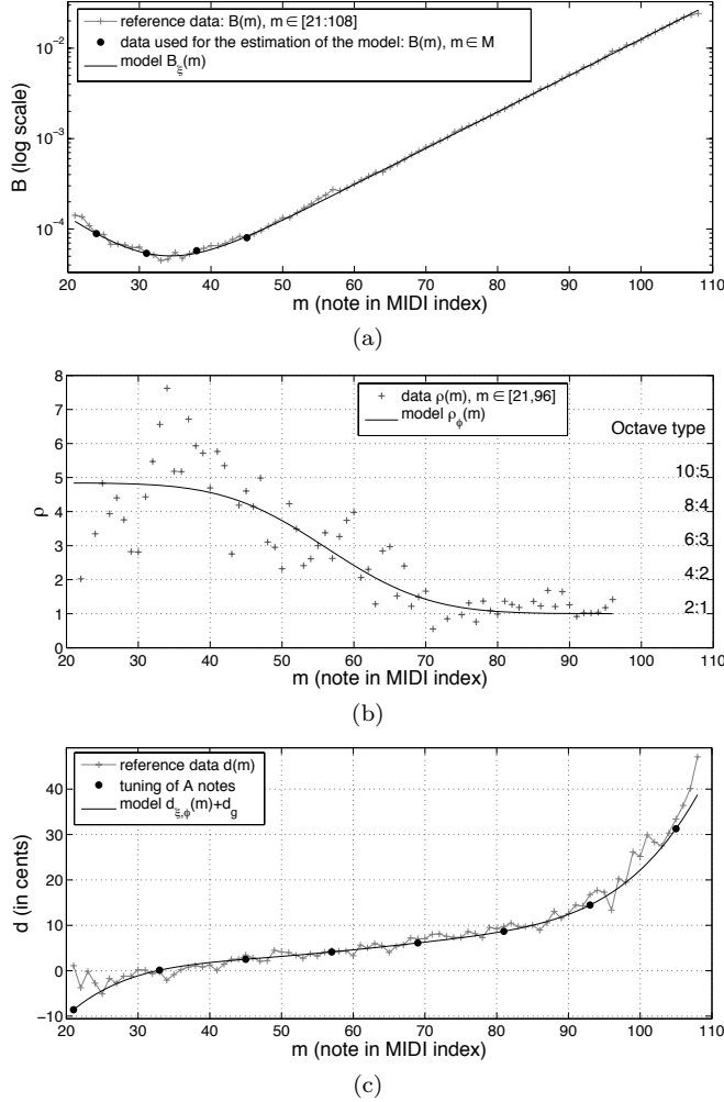
FIG. 7. RWC grand piano #3. (a) Inharmonicity coefficient B , (b) octave type parameter \rho , (c) deviation from ET along the whole compass. The data are depicted as grey '+' markers and the model as black lines.
