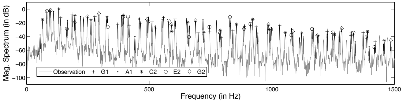
FIG. 6. Result of the algorithm for the analysis of the chord #1 (G1-A1-C2-E2-G2) of MAPS grand piano synthesizer.
