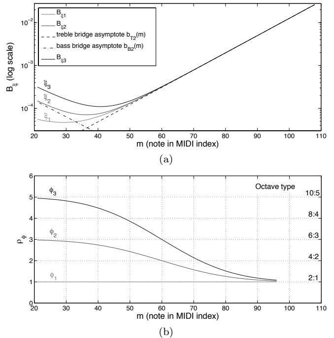
FIG. 1. Model for (a) inharmonicity coefficient B_\xi(m) and (b) octave type parameter \rho_\phi(m) along the compass for different values of the sets of parameters.
